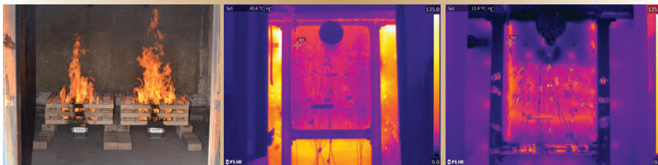
Fire at 4.5 minutes Ceiling temp: 150°C (302°F)
