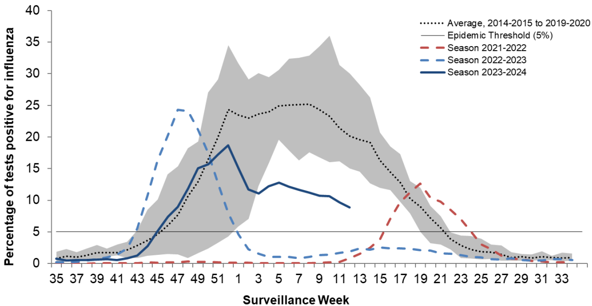
Figure 3 –Percentage of tests positive in Canada compared to previous seasons, week 2023-35 to 2024-12
