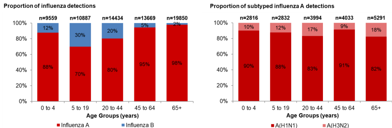
Figure 4 – Proportion of positive influenza specimens by type or subtype and age-group reported through case-based laboratory reporting, Canada, week 2023-35 to 2024-12
