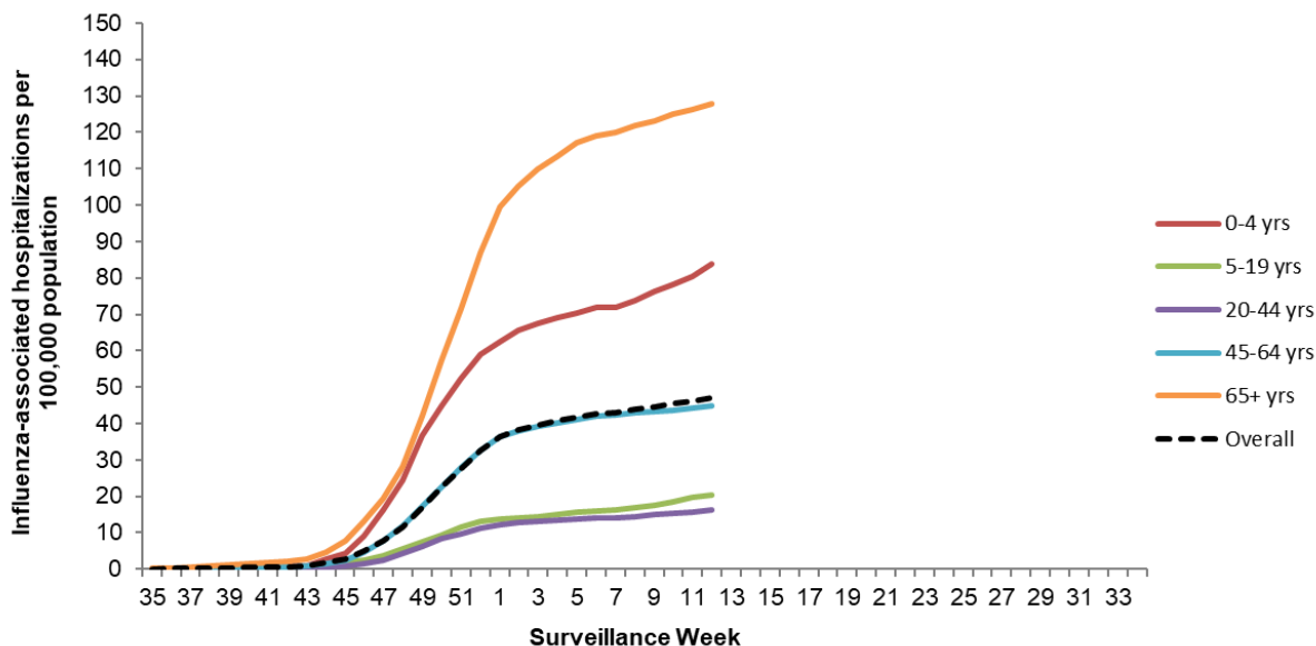
Figure 8 – Cumulative rates of influenza-associated hospitalizations by age-group and surveillance week, Canada, participating provinces and territories, week 2023-35 to 2024-12
