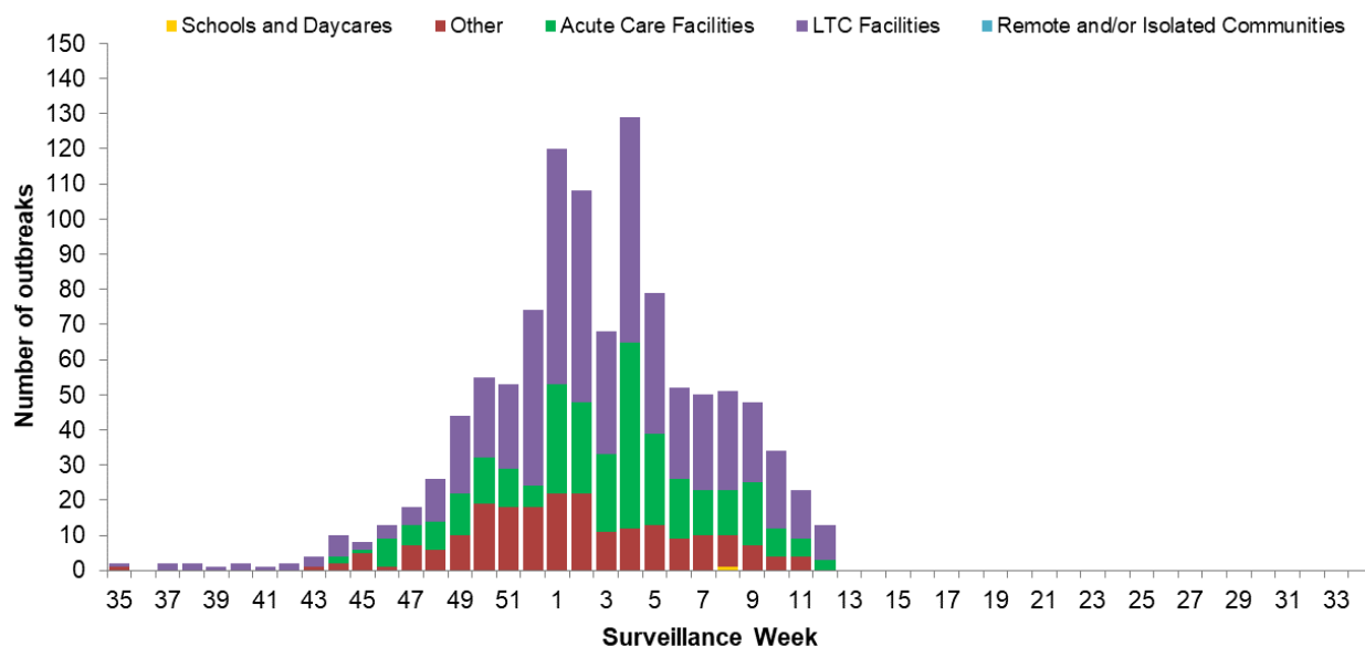
Figure 7 – Number of new outbreaks of laboratory-confirmed influenza by report week, Canada, weeks 2023-35 to 2024-12
