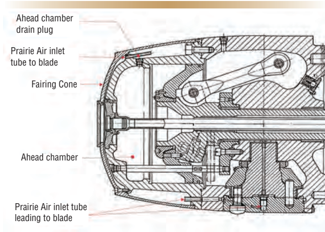
Propeller hub schematic.
