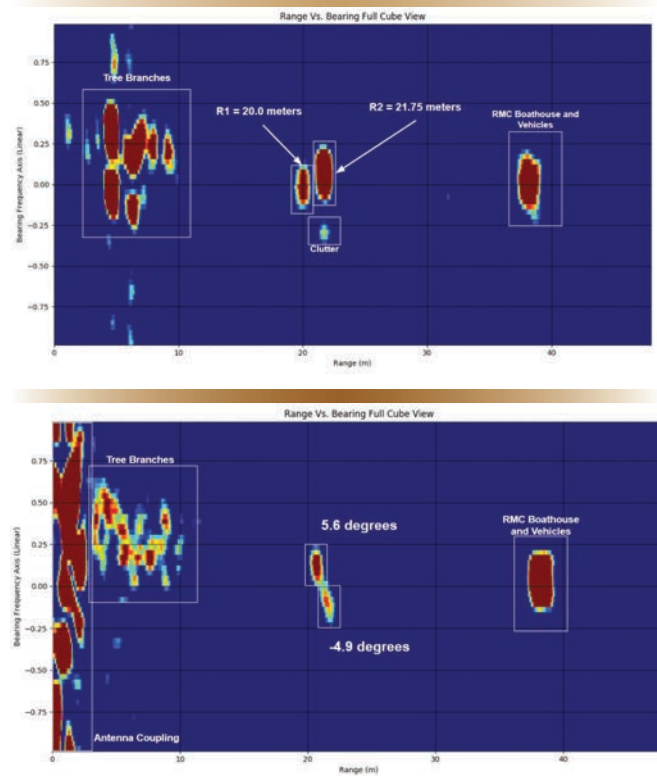
Figure 16. CDM MIMO radar range vs. bearing display, showing a range resolution of 1.75 m (top), and angular resolution of 10.5 degrees (bottom).
