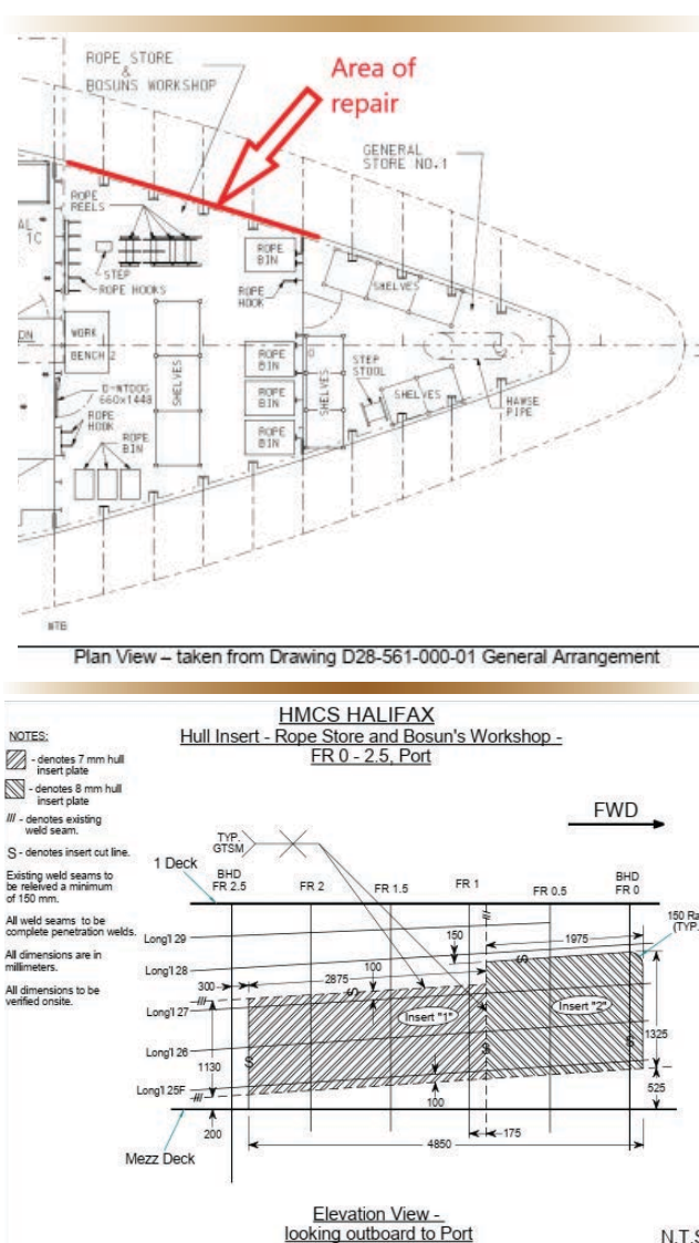
Figure 5. Schematics showing the placement of the two hull inserts.
