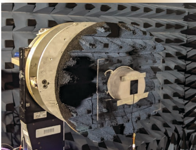
Figure 10. Tagolas 10-GHz ultra-wideband antenna in the anechoic chamber at RMC.
