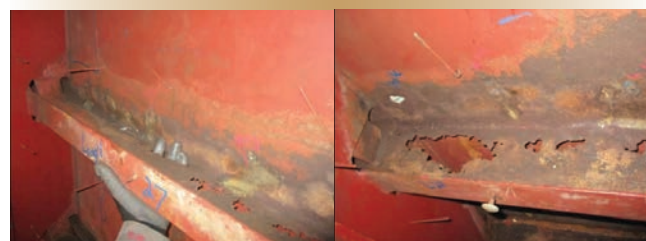
Figure 2. Holed and wasted sections of longitudinal.
