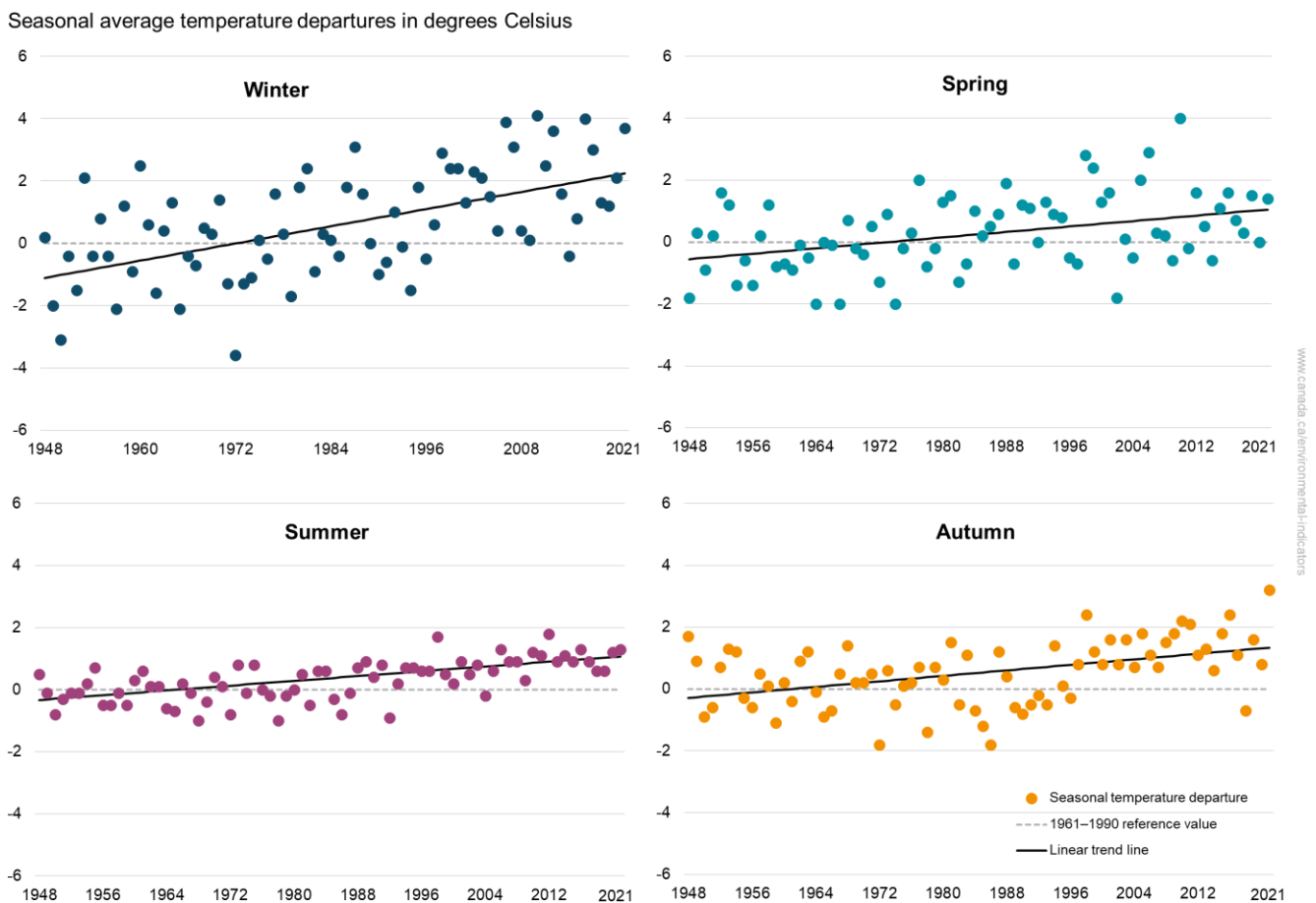
Figure 2. Seasonal average temperature departures compared with the 1961 to 1990 reference value, Canada, 1948 to 2021
