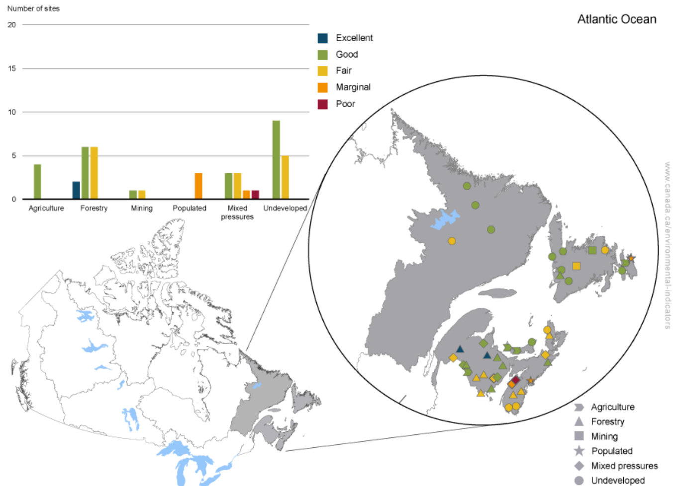
Figure 4. Water quality by land use category, Atlantic Ocean region, 2017 to 2019 period
