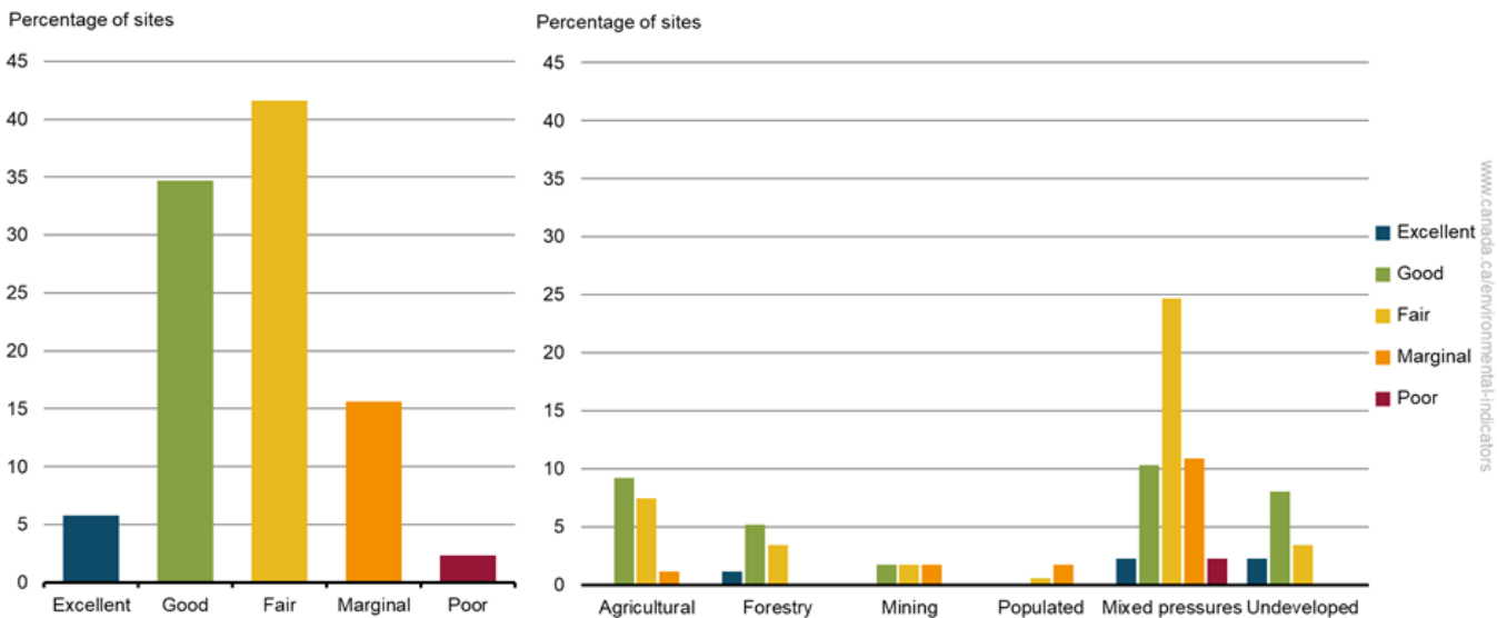
Figure 1. Water quality in Canadian rivers, national and by land use category, 2017 to 2019 period
