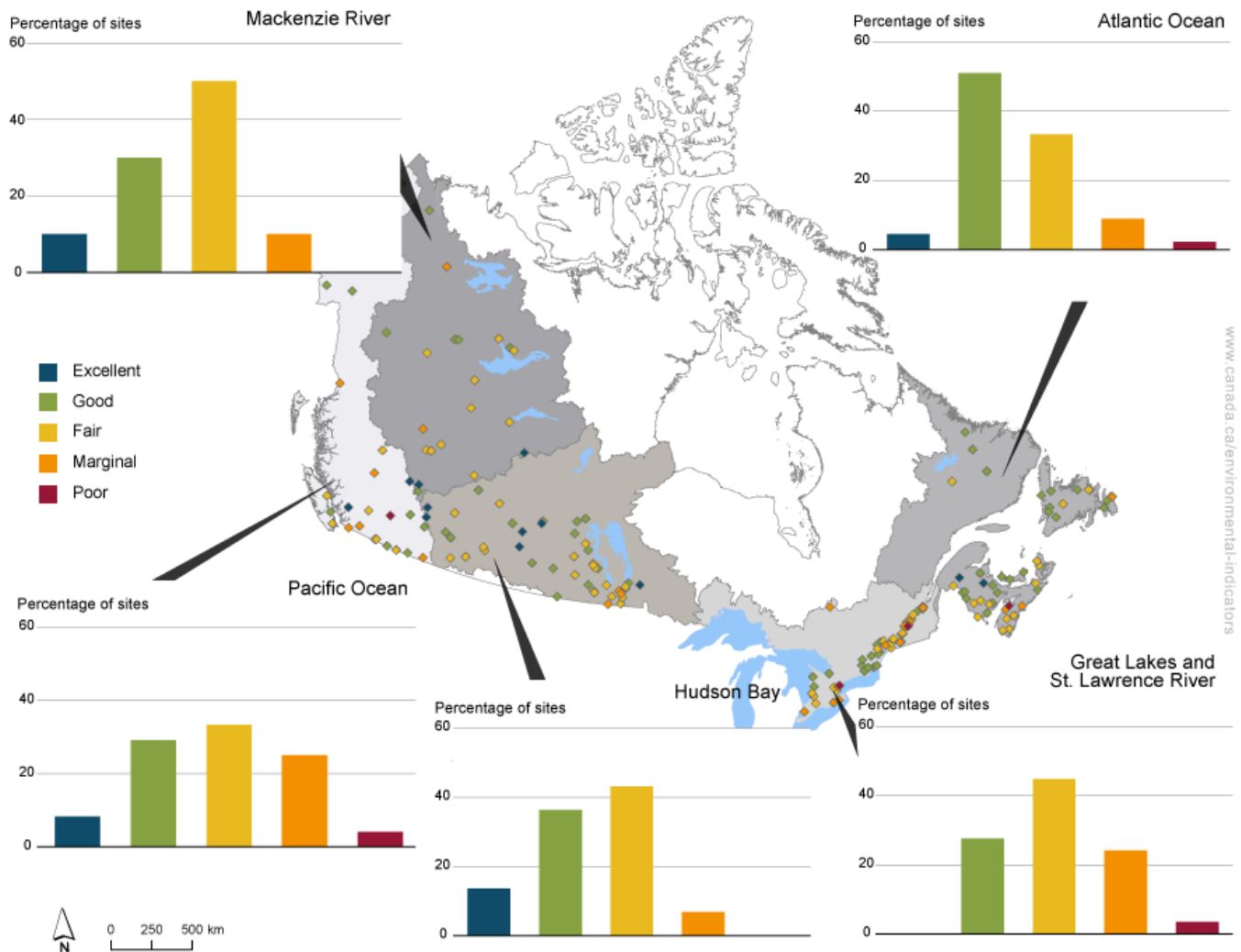
Figure 3. Regional water quality, Canada, 2017 to 2019 period
