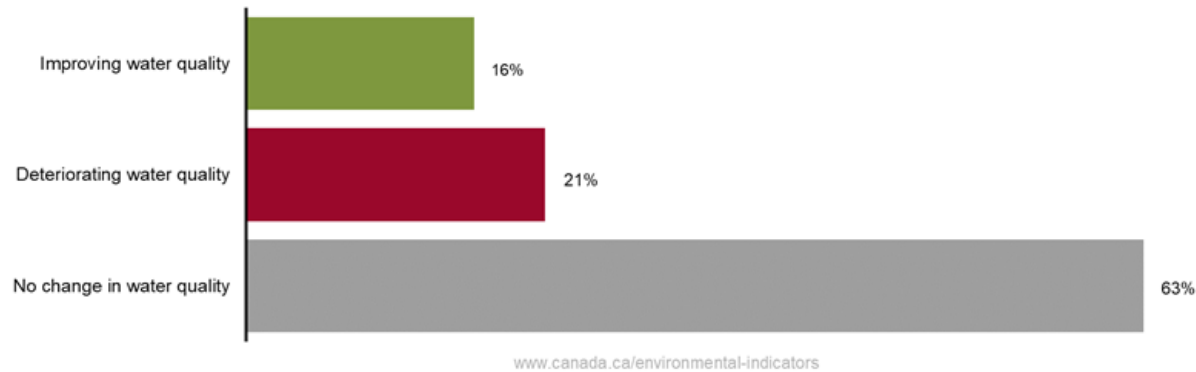
Figure 2. Trends in water quality, Canada, 2002 to 2019
