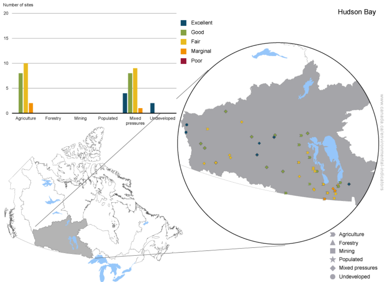
Figure 6. Water quality by land use category, Hudson Bay region, 2017 to 2019 period
