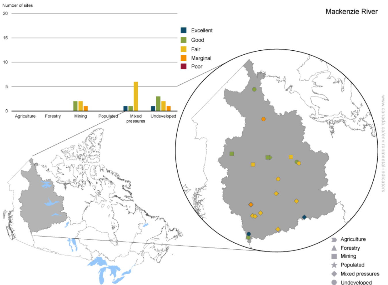
Figure 7. Water quality by land use category, Mackenzie River region, 2017 to 2019 period
