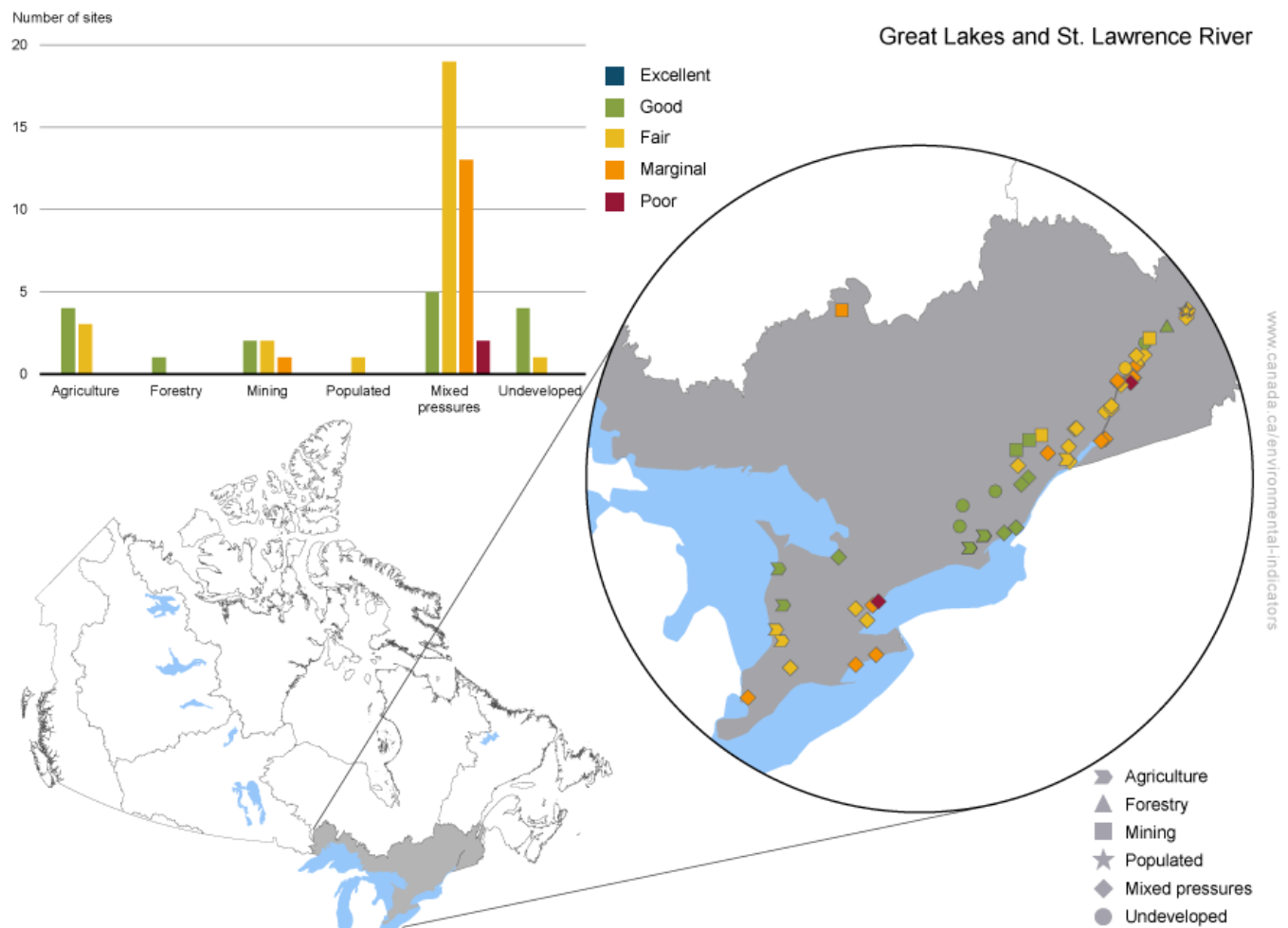
Figure 5. Water quality by land use category, Great Lakes and St. Lawrence River region, 2017 to 2019 period
