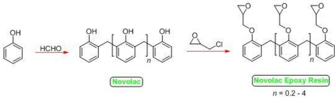
Figure 3-1. Representative structure of Novolac epoxy resin
