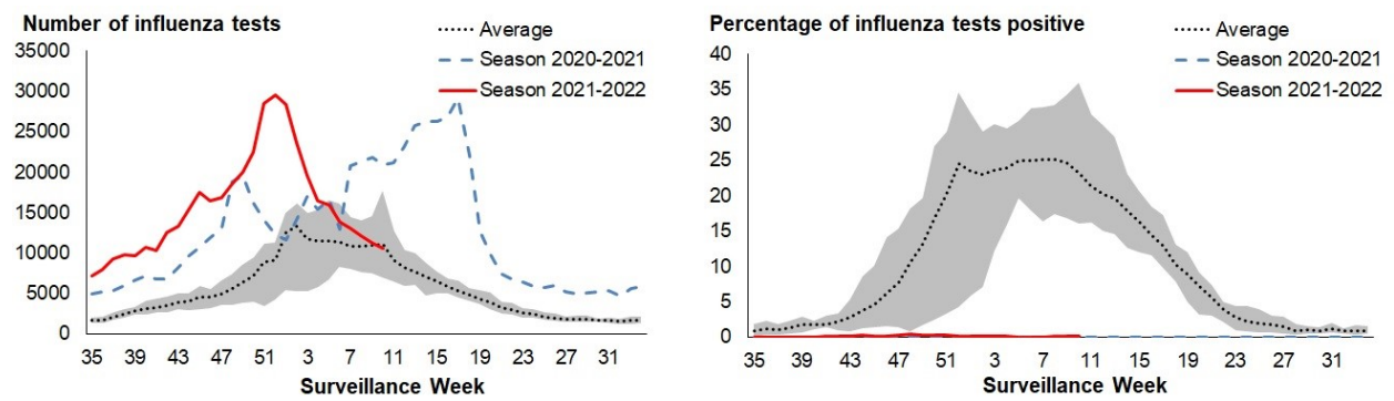
Figure 3 – Number of influenza tests and percentage of tests positive in Canada compared to previous seasons, week 2022-10
