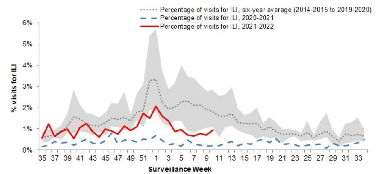
Figure 5 – Percentage of visits for ILI reported by sentinels by report week, Canada, weeks 2021-35 to 2022-10
