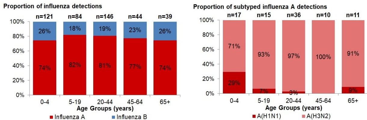
Figure 4 – Proportion of positive influenza specimens by type or subtype and age-group reported through case-based laboratory reporting, Canada, weeks 2021-35 to 2022-10
